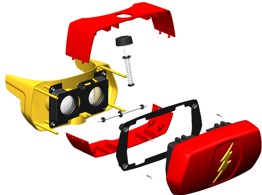
Exploded View
